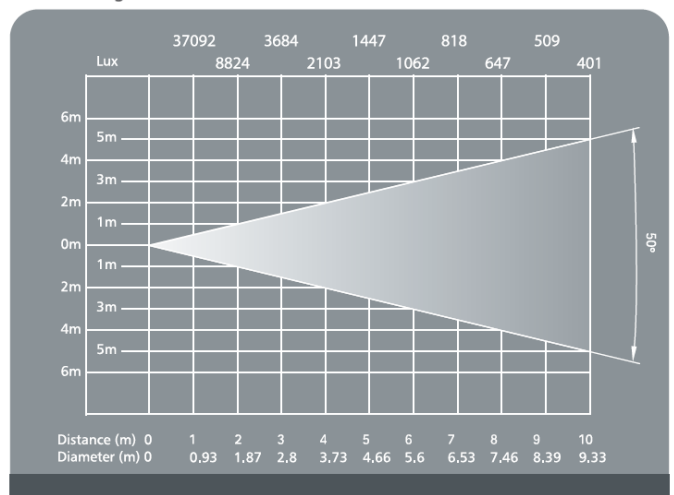
Beam angle 50°
