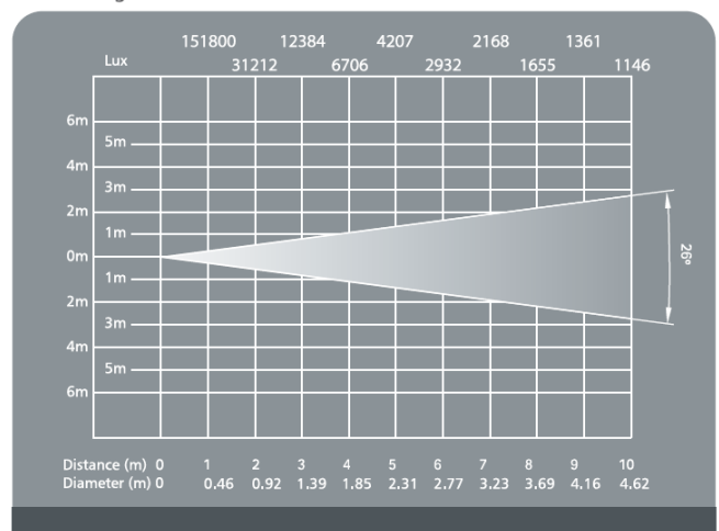
Beam angle 26°
