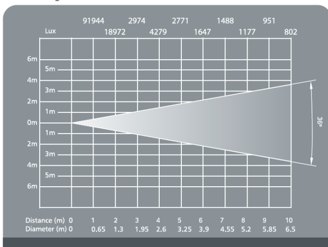
Beam angle 36°
